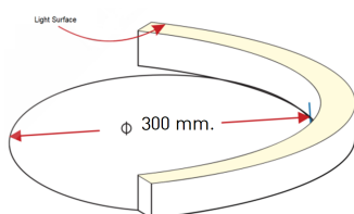
Horizontal bending
